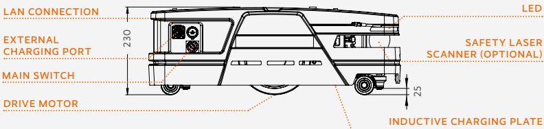
XS1 CORE SIDE VIEW
